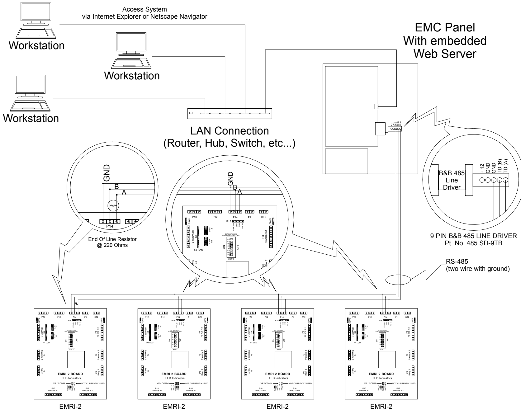
Stand Alone System EMRI-2 Board typical connections to EMC Panel
