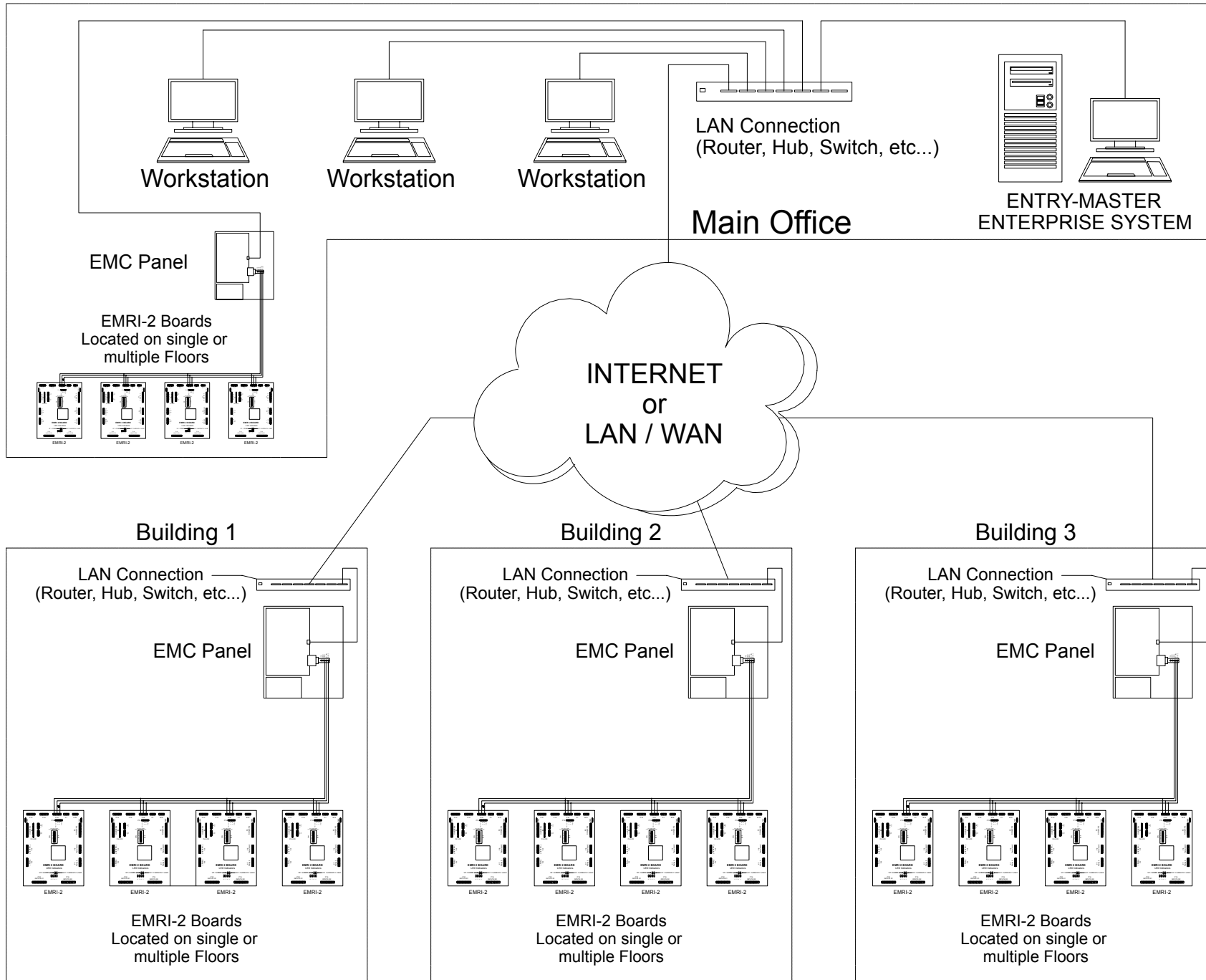
Entry-Master Enterprise System connected to multiple facilities via LAN, WAN, or INTERNET
